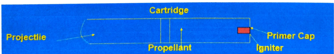
Propellant Train
