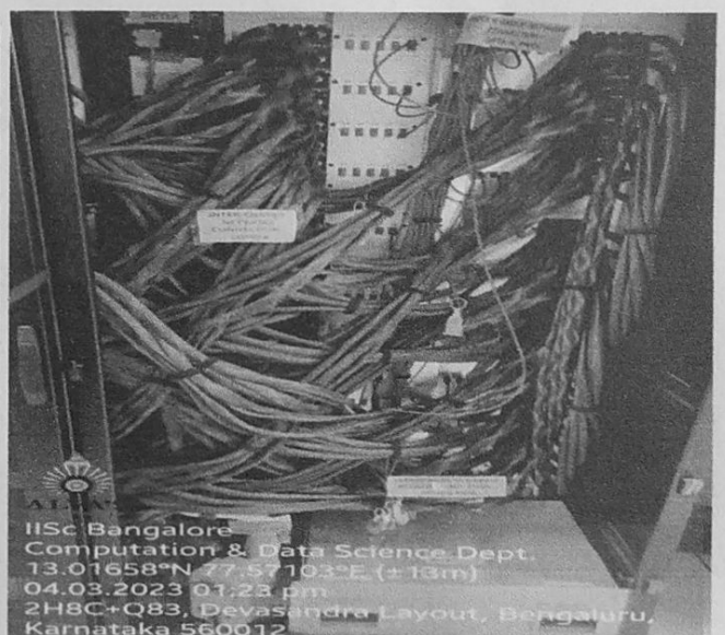
Super computer CRAY XC40, configuration chart and connections using copper and FC cables
